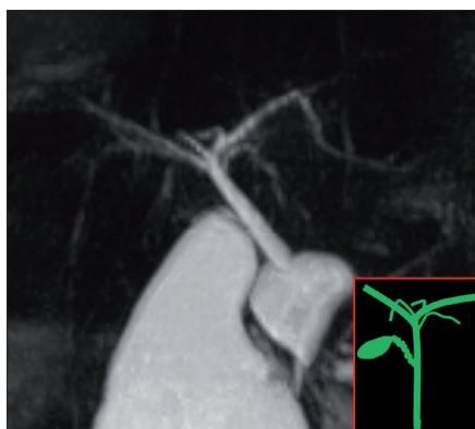
Figure 7. Novel Type 13: MRCP image with an illustration showing the trifurcation associated with right segmental duct draining into the left main biliary duct and left segmental duct draining into CHD.
