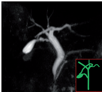
Figure 5. Novel Type 11: MRCP image with an illustration showing the trifurcation associated with right segmental duct draining into CHD.
