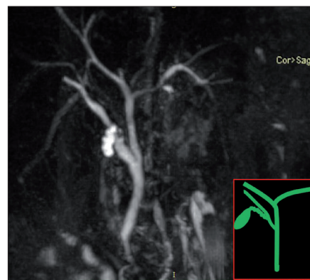
Figure 12. Novel Type 18: MRCP image with an illustration showing the accessory right segmental duct draining into CHD and cystic duct draining into this accessory right segmental duct.
