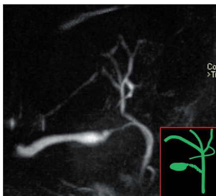
Figure 9. Novel Type 15: MRCP image with an illustration showing the trifurcation associated with right segmental duct draining into the left main biliary duct.
