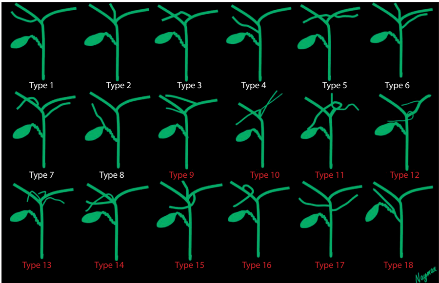
Figure 2. Intrahepatic bile duct variations. Types 1–8, previously classified types. Types 9–18, novel defined variants.
