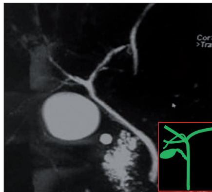
Figure 8. Novel Type 14: MRCP image with an illustration showing the trifurcation formed by three right segmental ducts.
