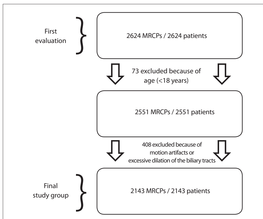
Figure 1. A flowchart showing the evaluation of the MRI data according to the exclusion criteria.
