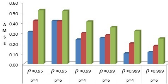
Figure 7.2. Bar graphs of different variance values of k_{AY2} for different p and \rho
