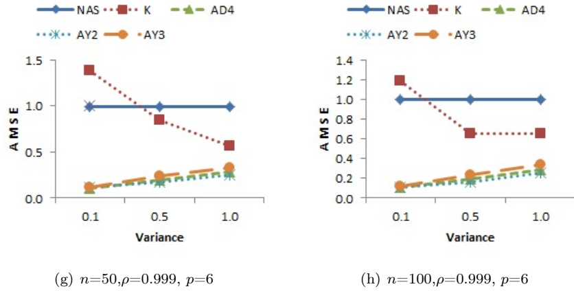
Figure 7.1. Comparison graphs of AMSE Values for selected k 's Variance ■ 0.1 ■ 0.5 ■ 1.0
