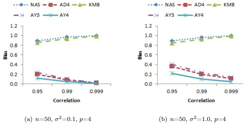
Figure 7.3. Comparison graphs of bias values with respect to different correlations for selected k 's
