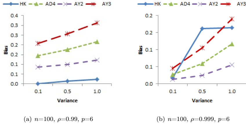
Figure 7.4. Comparison graphs of bias values with respect to different variances for selected k 's
