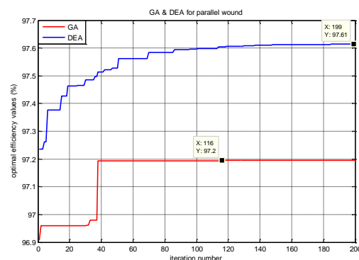
Figure 9. The convergence graphics of GA&DEA for parallel wound
