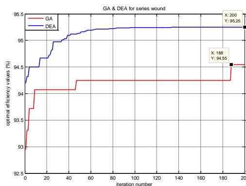
Figure 8. The convergence graphics of GA&DEA for series wound
