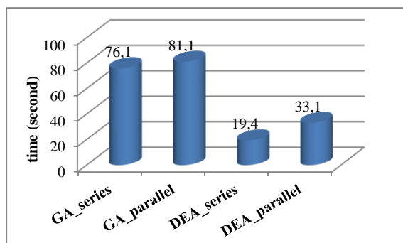
Figure 7. The convergence times of both algorithms
