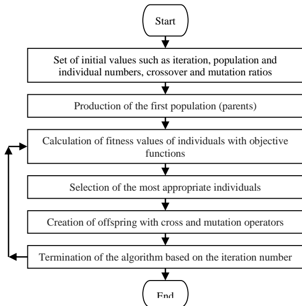
Figure 3. Flowchart of the genetic algorithm
