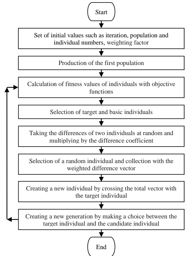
Figure 4. Flowchart of the differential evolution algorithm
