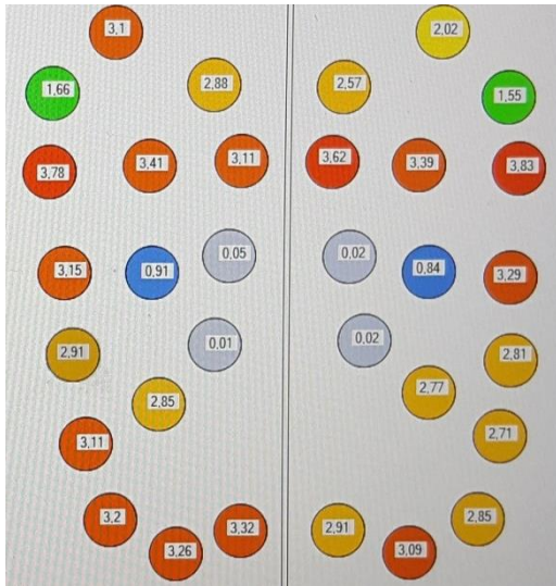
Fig 16. Average force generated by sensors during walking
